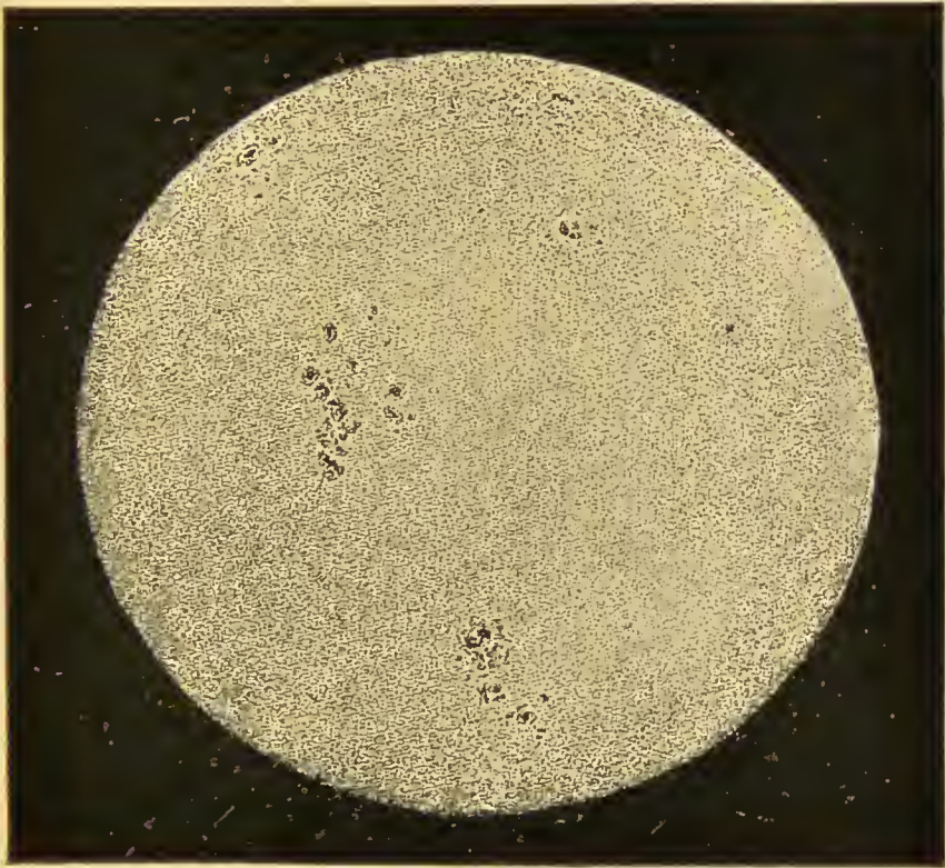
FIG. 43.—Sun spots, exceptionally numerous.
